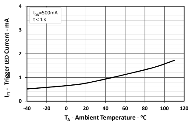
Fig. 5 Trigger LED Current vs. Ambient Temperature
